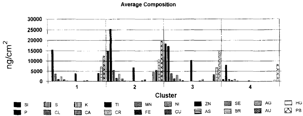
Fig. 2. Average elemental concentrations associated with each of the four clusters for the coarse mode aerosol.
