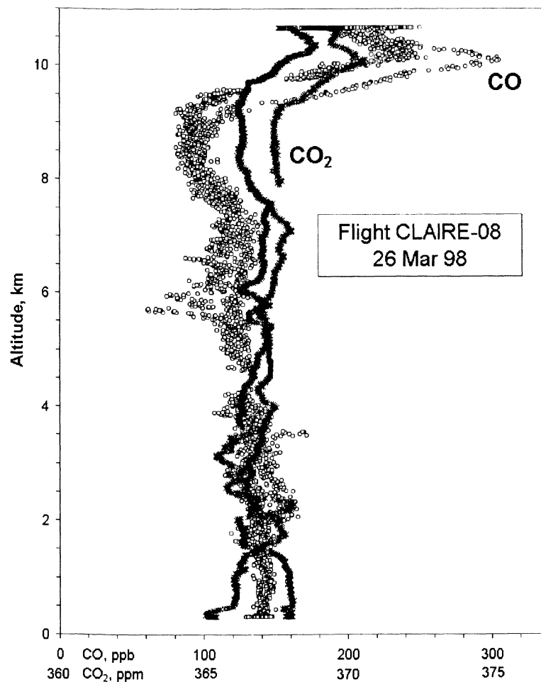
Figure 5. Vertical profiles of carbon monoxide (ppb) and carbon dioxide (ppm) observed during flight number 8 (March 26, 1998) over Suriname and Guyana.
