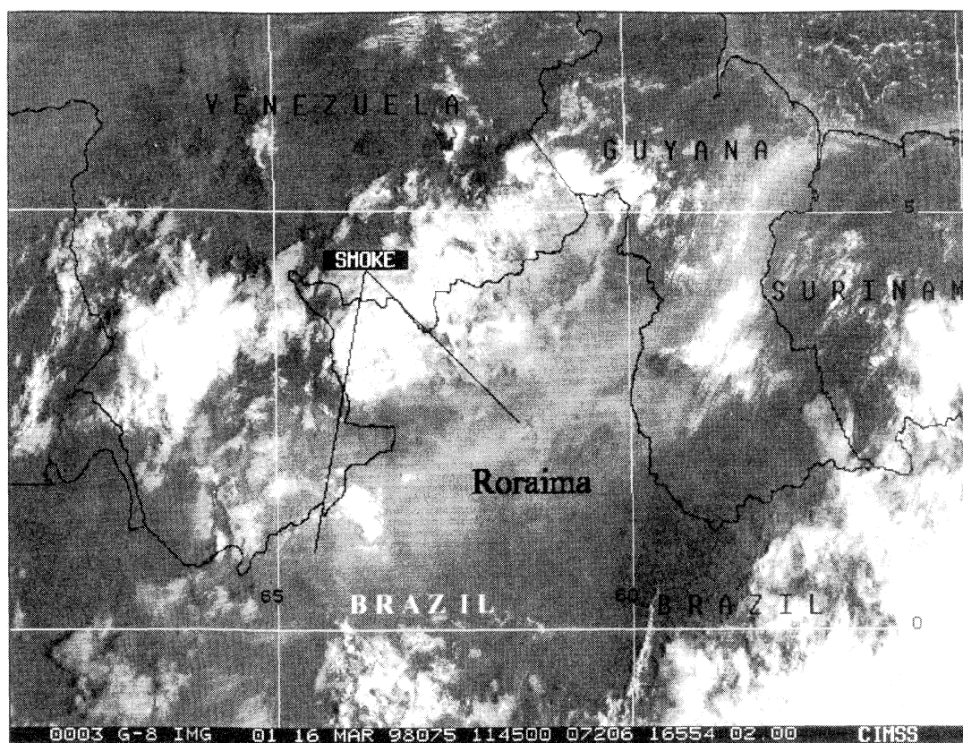
Figure 2. GOES-8 visible satellite image at 1145 UTC, March 16, 1998, showing the smoke produced by biomass burning over the Brazilian State of Roraima.
