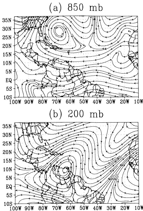
Figure 3. (a) Time average over the first three days (0000 UTC, March 16, to 0000 UTC, March 19, 1998) of the wind field at 850 mbar height and (b) time average over the last three days (0000 UTC, March 23, to 0000 UTC, March 26, 1998) of the wind field at 200 mbar height.
