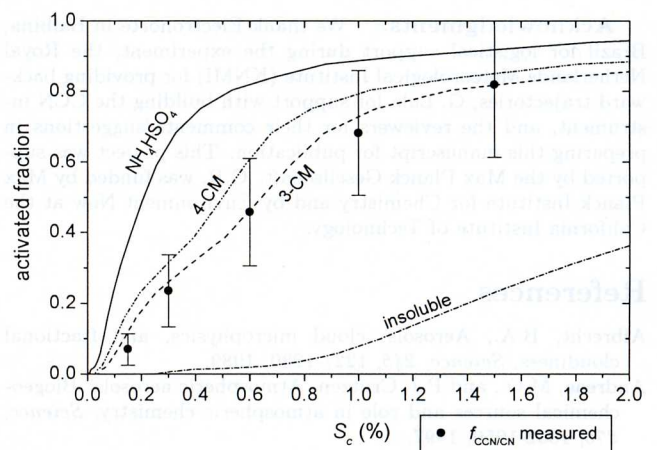
Figure 1. Fraction of aerosol expected to activate as CCN. The three-component (3-CM) example divides the aerosol mass into soluble inorganic ( \text{NH}_4\text{HSO}_4 ) and insoluble (inorganic and organic) components. The four-component model (4-CM) introduces the effect of 0.01 M dissolved organic carbon and the reduction of surface tension by 15%. Examples of \text{NH}_4\text{HSO}_4 and insoluble aerosol illustrate the limits of CCN activity based on measured number distributions.
