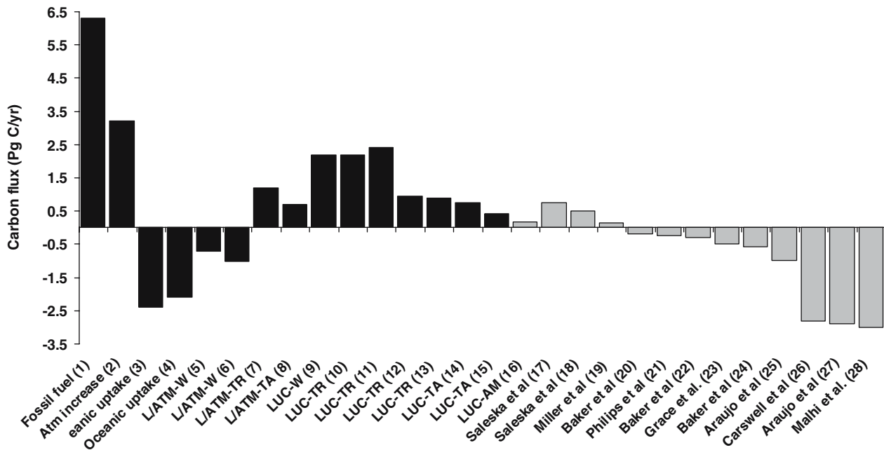
Fig. 7 Carbon flux from several sources. Positive numbers denote sources of carbon to the atmosphere and negative numbers denote an uptake of carbon from the atmosphere. L/ATM denotes a flux from the land to the atmosphere; LUC denotes a flux due to land use changes. W World; TR Tropics; TA Tropical America; and AM Amazonia. (1) Fossil fuel emissions (Schimel et al. 2001); (2) Atmosphere increase in CO 2 (Schimel et al. 2001); (3) Estimate of ocean uptake of CO 2 (House et al. 2003); (4) Estimate of ocean uptake of CO 2 (Houghton 2003); (5) Estimate of terrestrial sink of carbon (Houghton 2003); (6) Estimate of terrestrial sink of carbon (House et al. 2003); (7) Source of carbon from total tropical lands to the atmosphere estimated by inversion models (Gurney et al. 2002); (8) Source of carbon from tropical lands of the Americas to the atmosphere estimated by inversion models (Gurney et al. 2002); (9) Source of carbon from lands of the entire world to the atmosphere due to land use changes (Houghton 2003); (10) Source of carbon from tropical lands to the atmosphere due to land use changes (Houghton 2003); (11) Source of carbon from tropical lands to the atmosphere due to land use changes (Fearnside 2000); (12) Source of carbon from tropical lands to the atmosphere due to land use changes (Achard et al. 2002); (13) Source of carbon from
