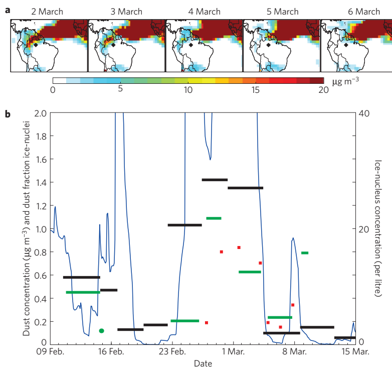
Figure 2 | Dust relation to ice-nucleus measurements. Dust concentrations during AMAZE-08. a , GEOS-Chem simulated dust from 2–6 March at 18 UTC. The field site, shown as a black diamond, typically fell near the edge of the plumes. Colour scale is saturated. b , Fine-dust concentrations from PIXE measurements (black rectangles; \mu\text{g m}^{-3} ; <2 \mu\text{m} , linewidths correspond to collection times) and GEOS-Chem simulations (blue line; \mu\text{g m}^{-3} ; <1.8 \mu\text{m} ). Also shown are the ice-nuclei fraction composed of dust (red squares) as determined from TEM-EDX and average ice-nucleus concentrations at -30^\circ\text{C} (green rectangles); linewidths designate sampling periods, although data were not necessarily collected continuously throughout these periods.
