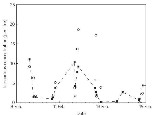
Figure 3 | Predicted ice-nucleus number concentrations. Measured (circles) and predicted (filled squares) ice-nucleus concentrations for a 6 day measurement period for CFDC processing temperatures of -18 to -31^\circ\text{C} . The filled squares represent the points of the calculations; the dashed lines are to guide the eye.
