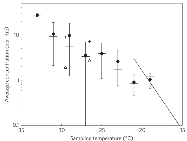
Figure 1 | Ice-nucleus number concentrations. Summary from all measurements collected during AMAZE-08. Data are binned in 2 °C increments and are presented as the mean (filled circle) and median (horizontal lines) ice-nucleus concentration as a function of temperature, corrected to standard temperature and pressure (0 °C and 1 atm). The variability in concentration (one standard deviation) at each temperature is also shown. For comparison, a global composite of ice-nucleus concentrations is shown (Fletcher 19 , solid line), as well as data for the mid-latitudes: Richardson et al. 20 (triangles) and DeMott et al. 18 (plus symbols).
