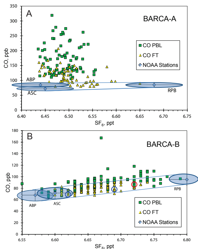
Fig. 4. Plot of CO from the flask samples against sulfur hexafluoride ( \text{SF}_6 ), which serves as a tracer of NH vs. SH air mass origin, for BARCA-A (A) and BARCA-B (B). The values measured simultaneously at the NOAA monitoring sites Ragged Point, Barbados (RBP), Arembepé, Brazil (ABP), and Ascension Island (ASC) are shown for reference. The red circle in panel (B) indicates a sample of PBL inflow off the Brazilian coast, the blue circles indicate samples of FT inflow.
