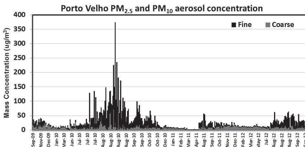
FIGURE 5. Time series of fine, coarse and PM 10 aerosol mass concentration for the Porto Velho monitoring station. Biomass burning impacts are easily observed during the dry season, especially for 2010, a very dry year in Amazonia.
