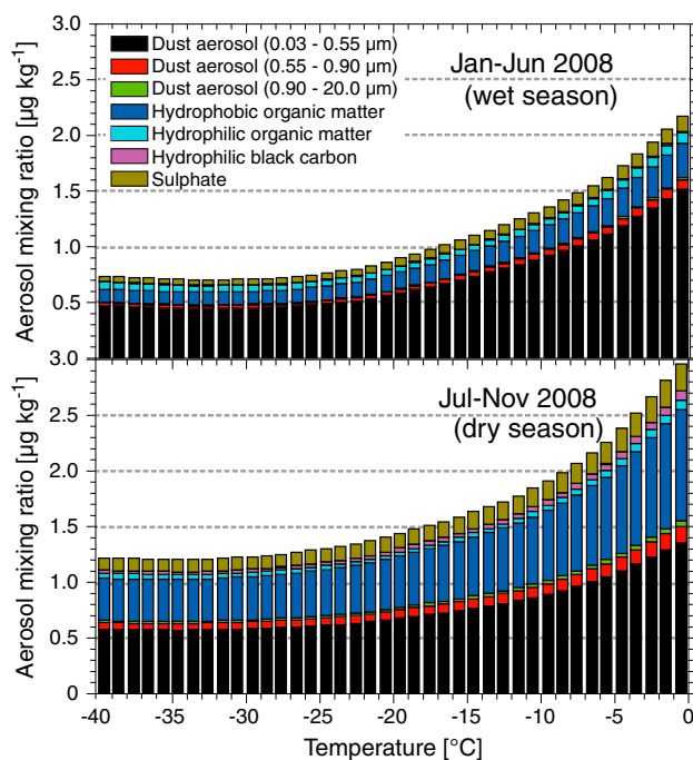
Figure 3. Seasonal profiles of aerosol mass mixing ratio of seven different aerosol species taken from the MACC reanalysis averaged over nine grid points closest to the observation site.
