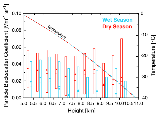
Figure 2. Mean (circles), median (center of boxes), and 25/75 percentiles (bottom and top of boxes) of the particle backscatter coefficient at 532 nm wavelength for the wet and dry season obtained from Polly XT observations as described in Baars et al. [2012]. Mean GDAS1 temperature profiles for both seasons are shown in addition.
