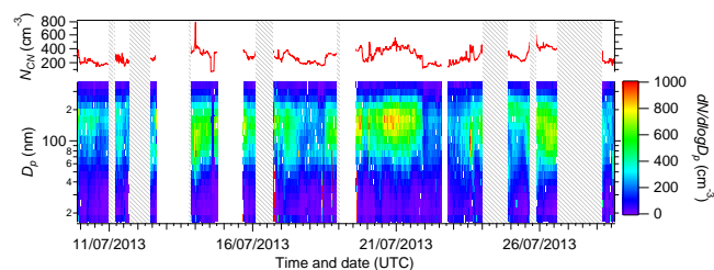
Figure 4. The time series of total particle counts (integrated from size distributions; top panel) and particle number size distribution (bottom panel). Shaded areas represent pollution episodes removed from the data. Any other gaps are due to instrument downtime.
