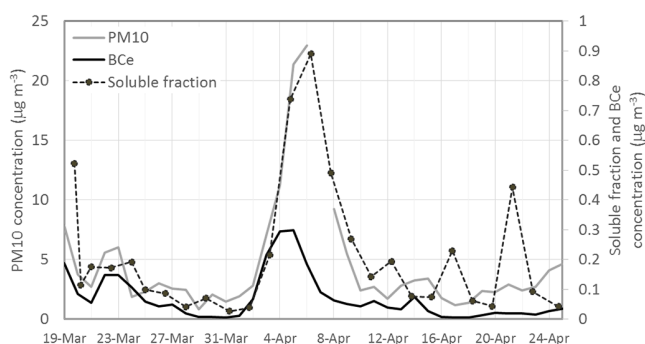
Figure 2. Time series of PM 10 mass concentration, integrated from size distribution measurements (size range: 0.3–10 μm); black carbon equivalent (BC e ) concentrations; and total concentration of particle soluble fraction.
