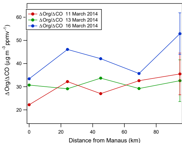
Figure 8. \Delta_{\text{org}}/\Delta_{\text{CO}} measurements in the plume as a function of distance from Manaus for 11, 13, and 16 March 2014. A representative error bar is shown for each set of measurements. Mean wind speeds were 5.8, 7.3, and 4.6 \text{m s}^{-1} on 11, 13, and 16 March, respectively. Collectively, the data capture approximately the first 4–6.5 h of the plume aging.
