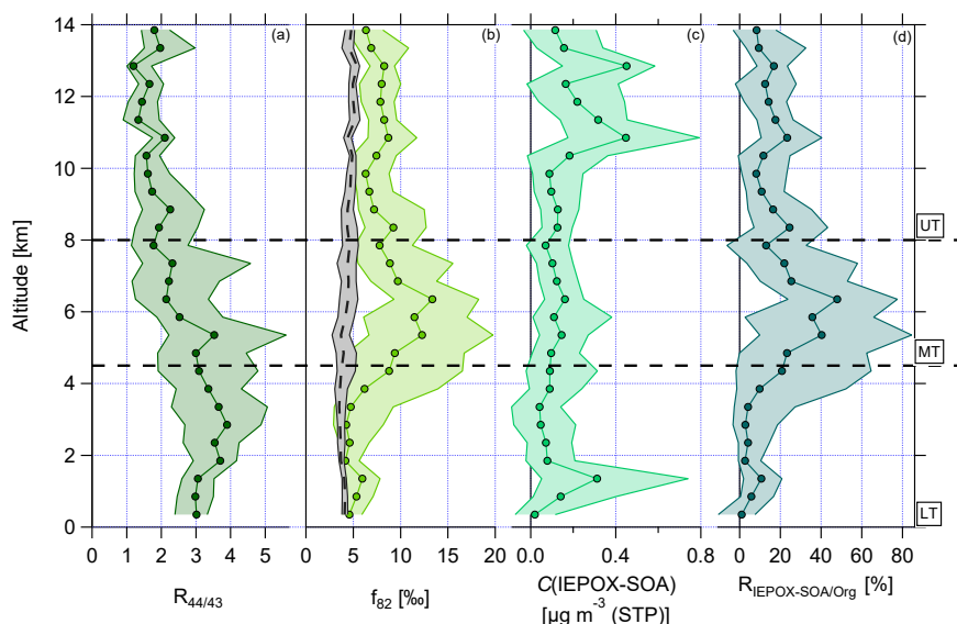
Figure 5. Vertical profiles with medians and interquartile ranges of (a) R_{44/43} , (b) f_{82} , (c) C(\text{IEPOX-SOA}) , and (d) R_{\text{IEPOX-SOA/Orig}} . Horizontal dashed lines indicate divisions into the LT with BL, MT, and UT. The vertical dashed line in (b) presents the calculated median background values f_{82}^{\text{Bg}} with interquartile ranges using Eq. (3). This equation is valid for areas with strong monoterpene influence (Hu et al., 2015, Appendix A).
