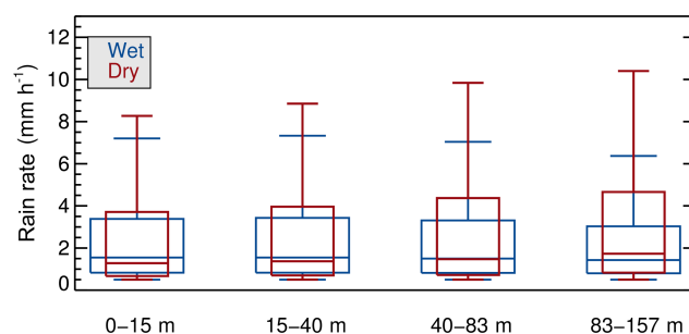
Figure 13. Wet and dry season rainfall rate (RR) box plots for different topography classes. Each box represents the 25 to 75 % populations, and the line inside the box represents the median value. The line represents the remaining population.
