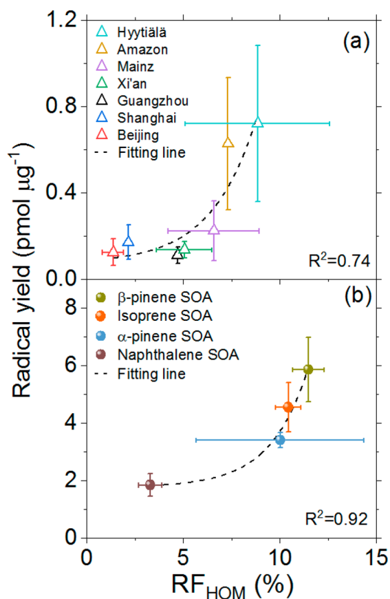
Figure 6. Correlation of particle mass normalized radical yield with relative ion number fraction of HOMs associated with ambient fine PM (a) and laboratory SOA (b). The error bars represent the standard deviation of measurement from replicates.
