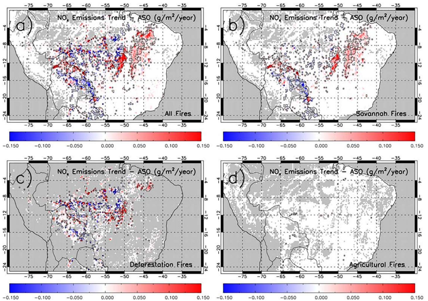
Figure 3. Trends in GFED \text{NO}_x ( \text{g}/\text{m}^2/\text{year} ) ASO total emissions between 2005 and 2016 for (a) all fires, (b) savannah fires, (c) deforestation fires, and (d) agricultural fires. Black polygon-outlined regions indicate significant trends above the 90% CL.
