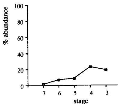
Fig. 6. Relative abundance of metal-rich particles as a function of particle size.
