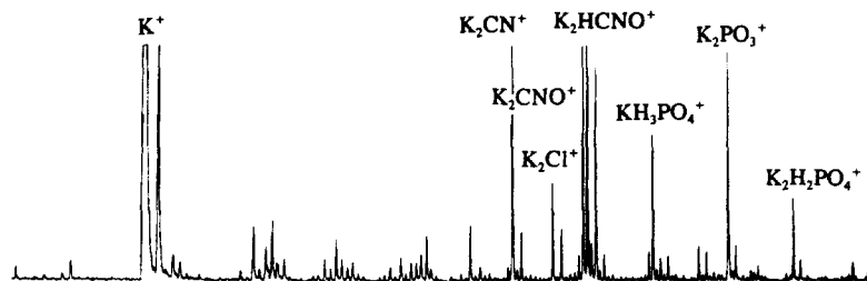
Fig. 4. Representative positive mode spectrum of a potassium-rich particle.
